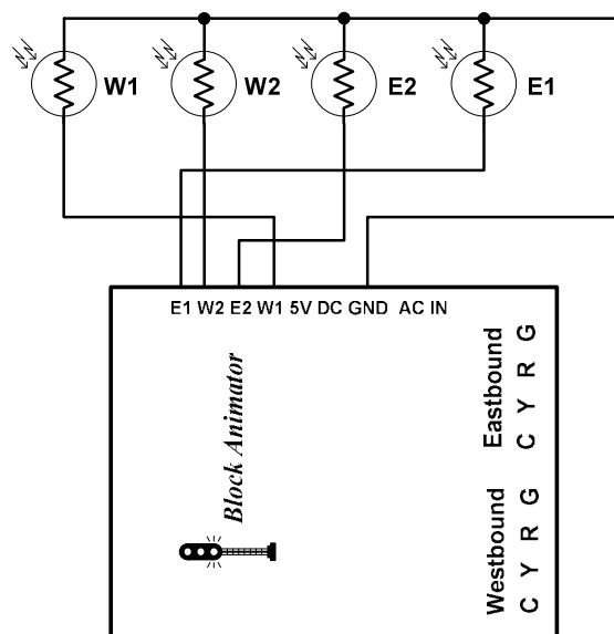
Figure 4 – photocell wiring
