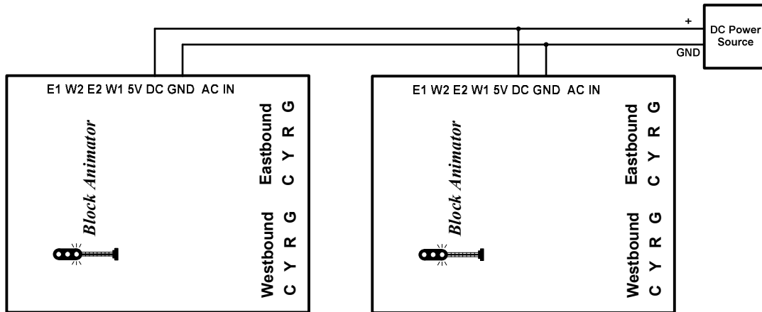
Figure 5 – DC power
