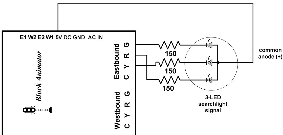
Figure 2 – 3-LED searchlight signal
