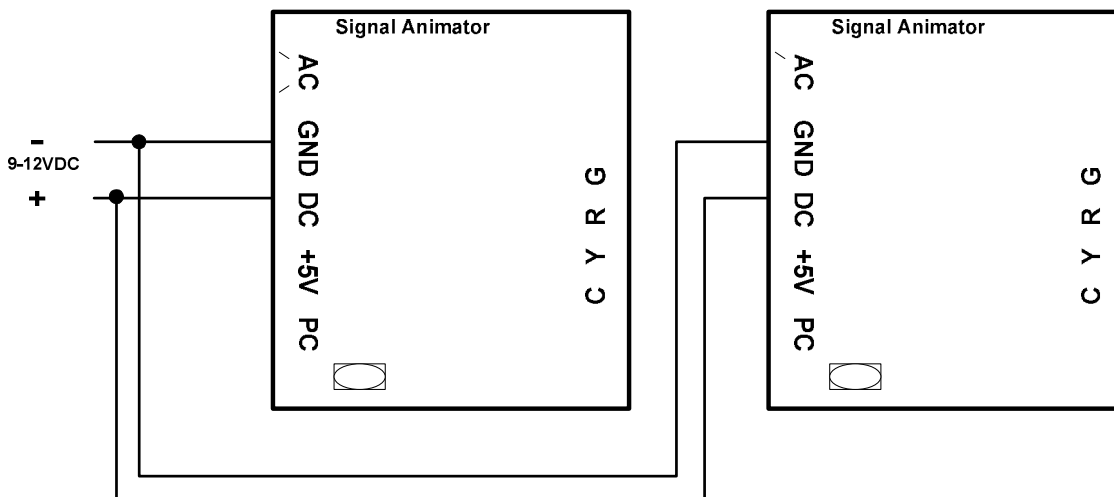
Figure 9 – DC power
