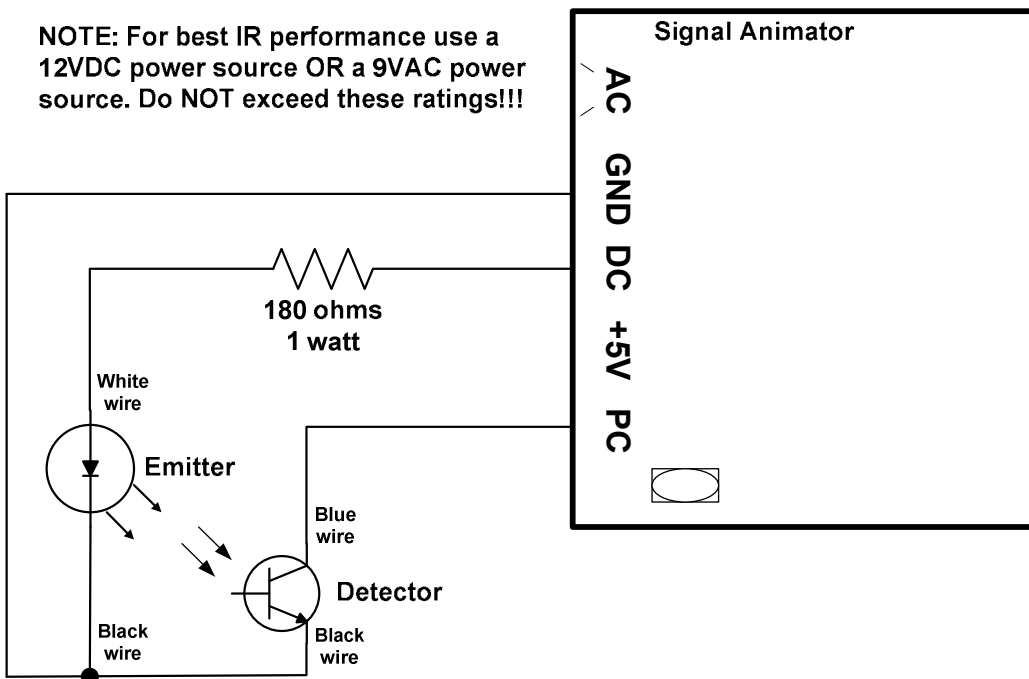
Figure 7 – IR component wiring
